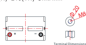
Terminal Dimensions
