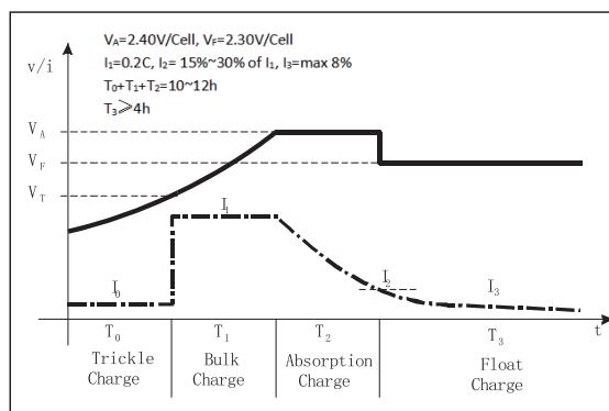
Charging characteristic
