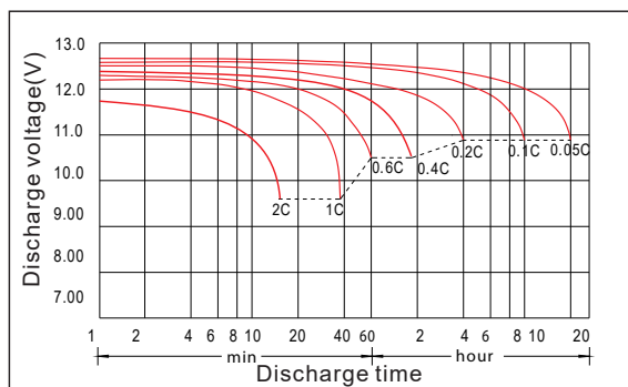
Discharge characteristic
