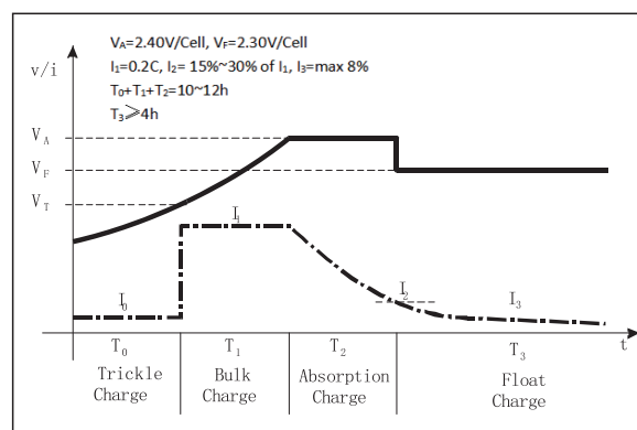
Charging characteristic
