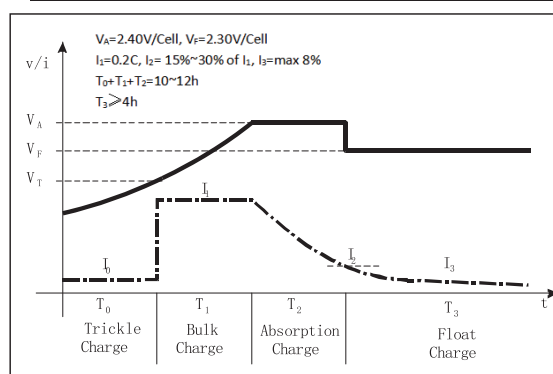
Charging characteristic
