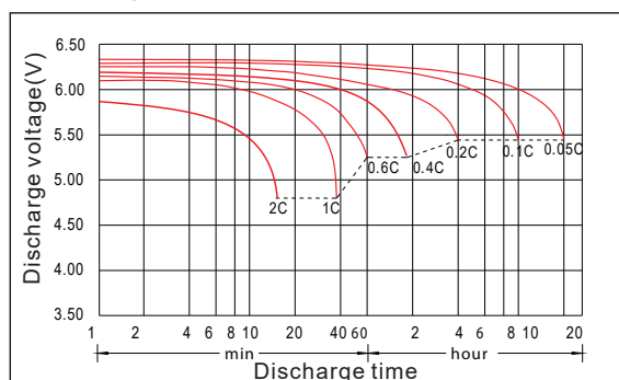
Discharge characteristic
