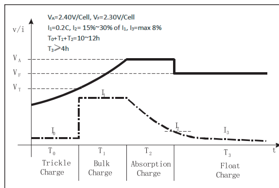
Charging characteristic
