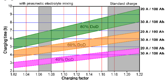
Charging times with IUla-characteristics in hours for PzS batteries at 30 °C
