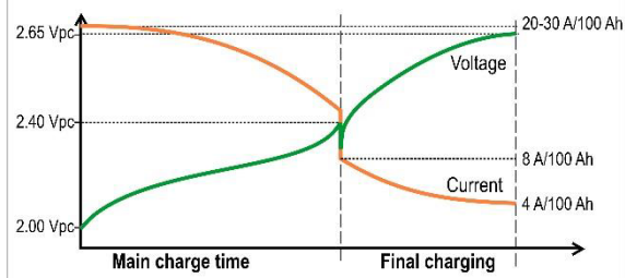
IUla –characteristics for flooded batteries
